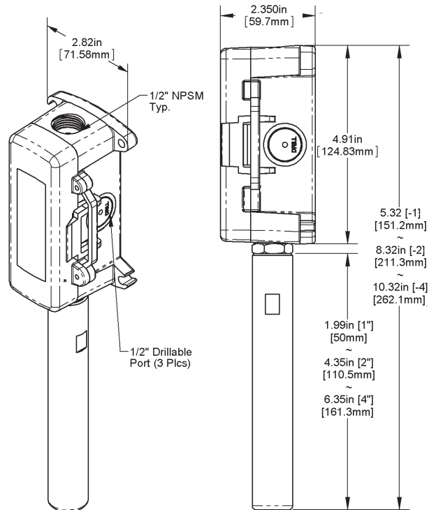
BAPI-Box 2 (BB2)
