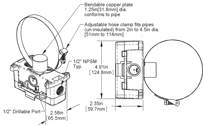
Clamp-On Strap BAPI-Box 2 (BB2)
