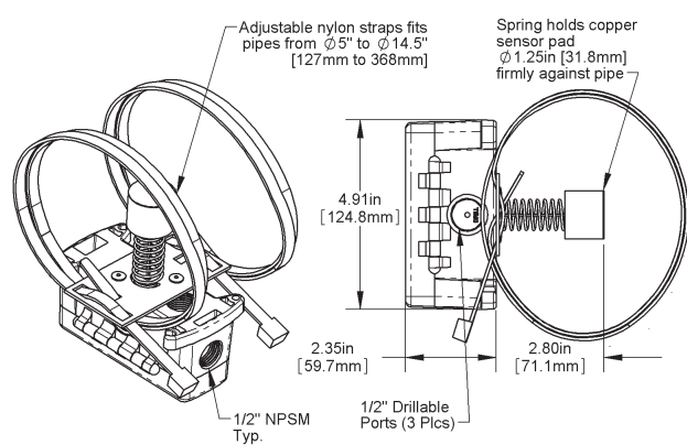
Spring-Loaded Strap BAPI-Box 2 (BB2)
