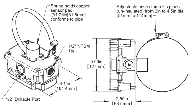
Clamp-On Strap BAPI-Box (BB)
