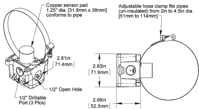
Clamp-On Strap BAPI-Box 4 (BB4)
