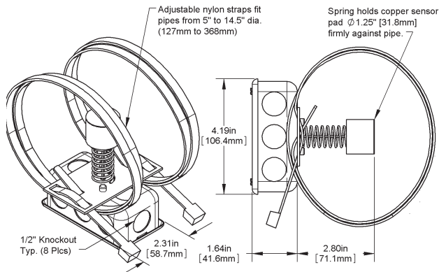
Spring-Loaded Strap J-Box (JB)
