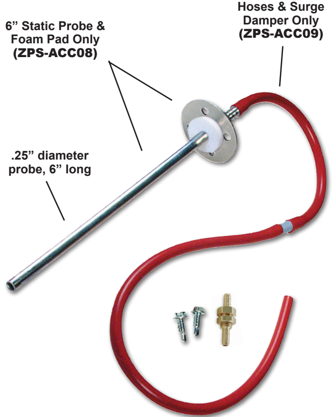
Static Pressure Probe Assembly, 6" (ZPS-ACC07)
