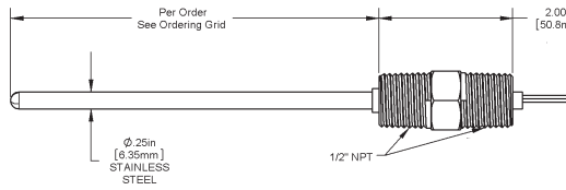
Immersion Probe without Enclosure
