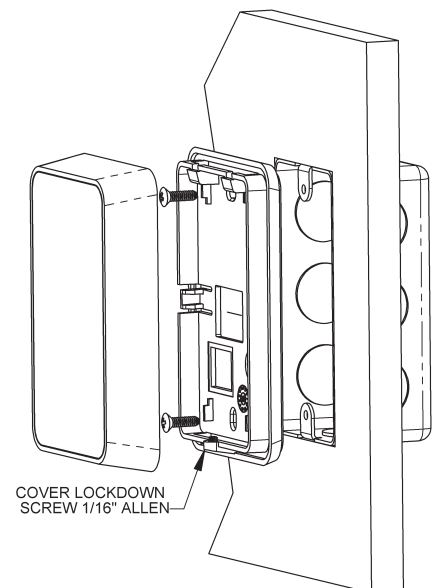
Fig. 2: BAPI-Stat “Quantum” J-Box Mounting
