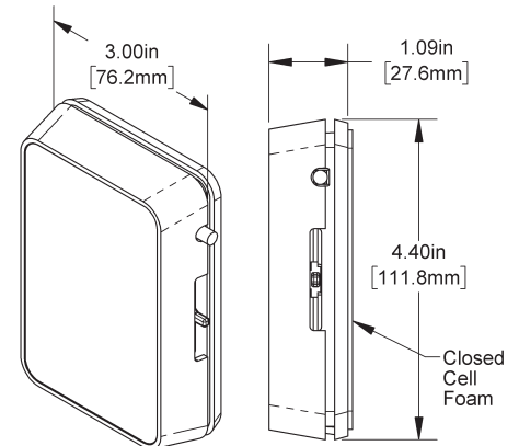
Fig. 1: BAPI-Stat “Quantum” Room Sensor without Display and included screw pack.
