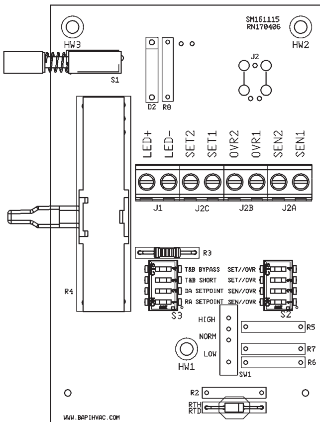
Fig. 3: Circuit board
