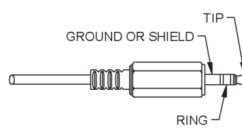
Fig. 6: C35 Comm. Jack (3.5mm plug shown for clarity)
