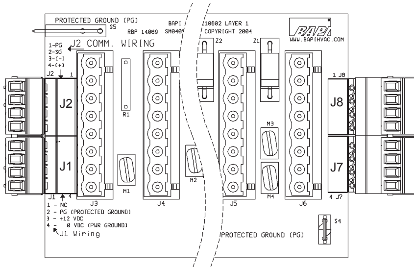
Fig. 3: RBPCX and RBPCX2 Wiring
