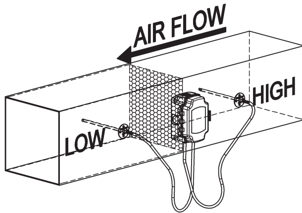
Fig. 13: Measuring duct air filter pressure drop with pressure transmitter and two static pressure probes.
