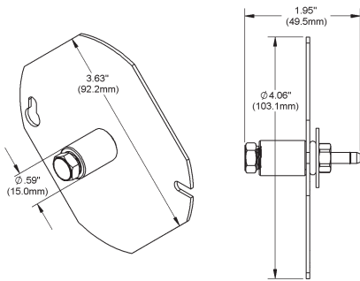
Fig. 6: Ceiling Mount Cover (ZPS-ACC05)
