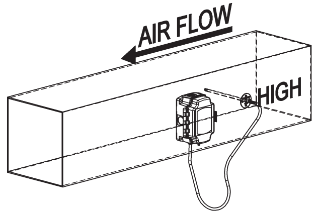
Fig. 14: Measuring duct static pressure with pressure transmitter and static pressure probe
