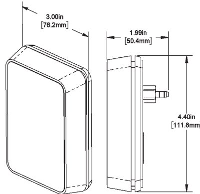
Fig. 10: BAPI-Stat "Quantum" (ZPS-ACC04) with standard mounting base
