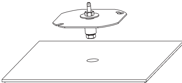
Fig. 15: Exploded view drawing of ceiling static pressure pickup port, BAPI ZPS-ACC05, showing how to mount in ceiling tile.
