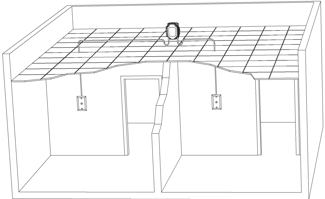
Fig. 12: Measuring static pressure differences between two rooms using two BAPI ZPS-ACC01 stainless steel wall plates and a BAPI ZPS Pressure Transmitter.
