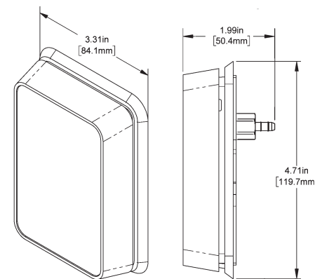
Fig. 11: BAPI-Stat "Quantum" (ZPS-ACC04-60) with 60mm mounting base to fit European wall boxes and junction boxes with 60mm mounting centers
