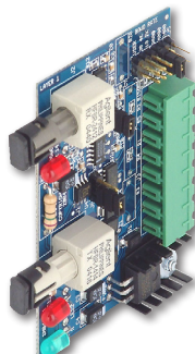
FOX - RS-485 Fiber Optic Transceiver (p. H24)
