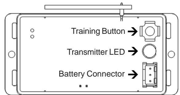
Fig 2: Transmitter Module
