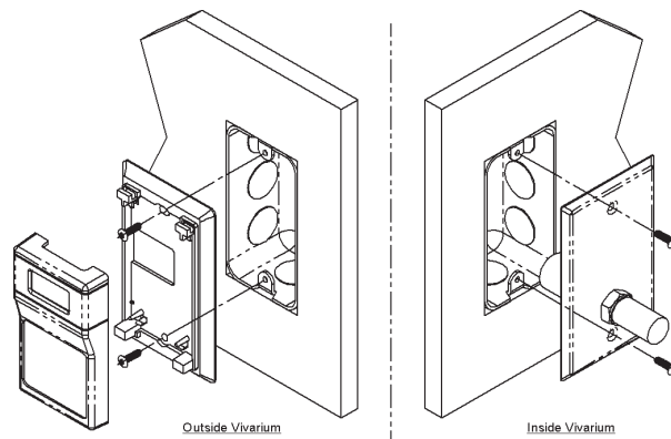
Figure 3: Display Unit & Vivarium Sensor Plate Mounting on Opposite Sides of the Same Wall.
