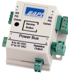
Resistance Output Module BA/ROM-102
